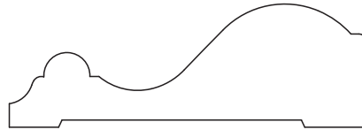
CCAS-874 1-1/8 X 3-1/2
